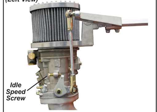
Figure 1 (Left View)
